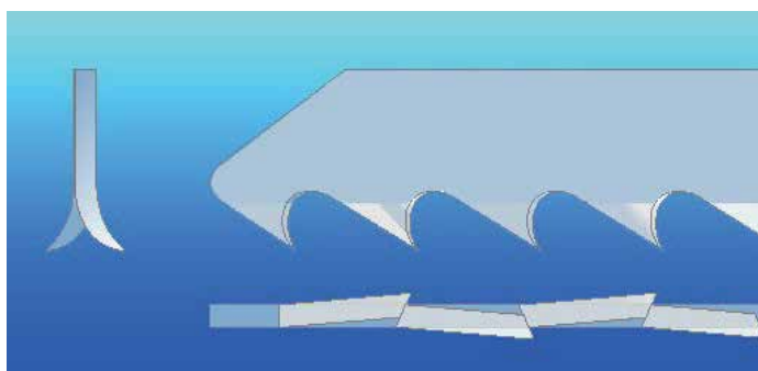
Ground and taper ground teeth
