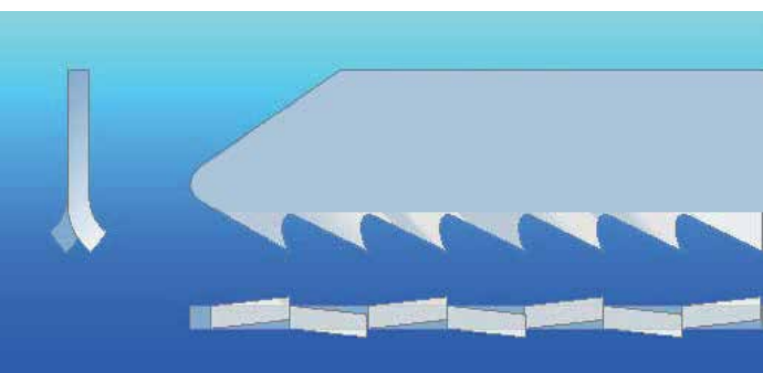
Milled and wavy set teeth
