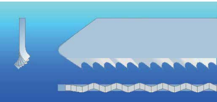
Milled and wavy set teeth
